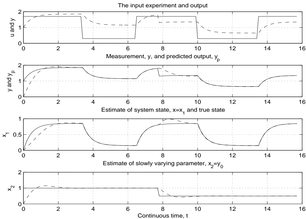
Figure 1: Simulation of the system in Example 7.1 with the state estimator in parallel. Butterworth observer polynomial with gain as in Equation (77).
