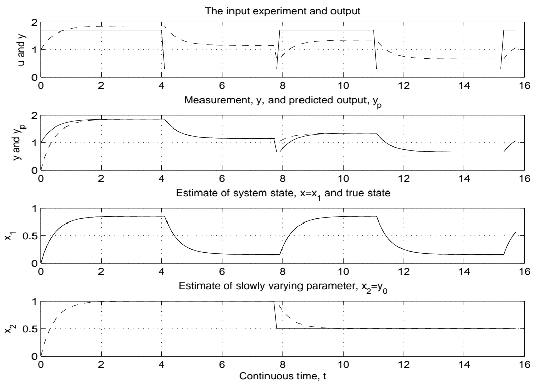
Figure 2: Simulation of the system in Example 7.1 with the state estimator in parallel. Observer polynomial with double time constants and gain as in Equation (78).
