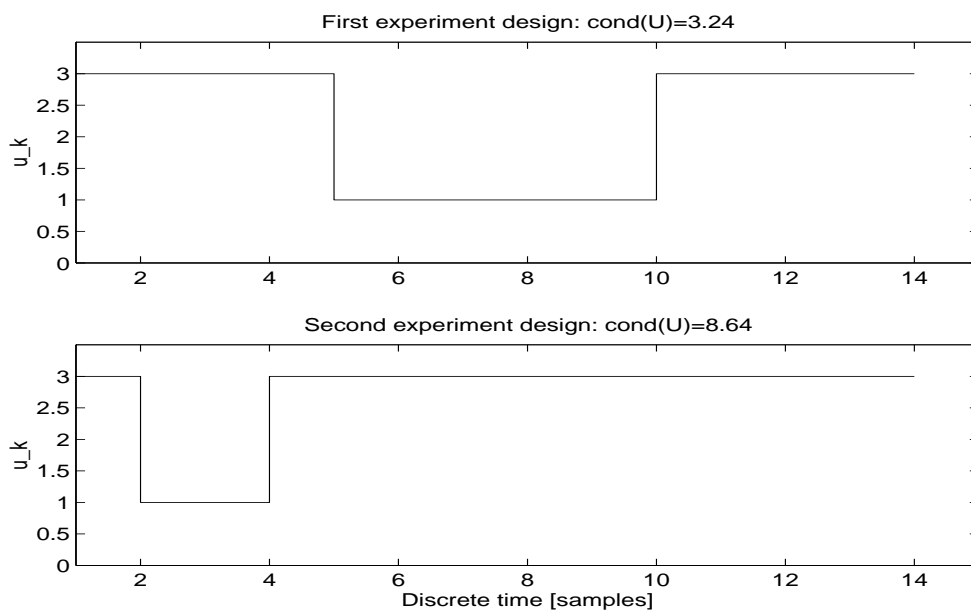
Figure 11.3: Illustration of two different binary input signal design. The design in the upper part has a condition number \text{cond}(U_{15}) = 3.236 and the design in the lower part \text{cond}(U_{15}) = 8.645 . The input design in the upper part is better conditioned for identification of a 5th ( n = 5 ) order dynamic model compared to the input design in the lower part. See example 11.1 for details.
