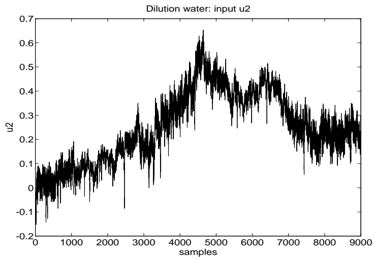
Figure 5.4: Flow of Dilution water, u_2 .
